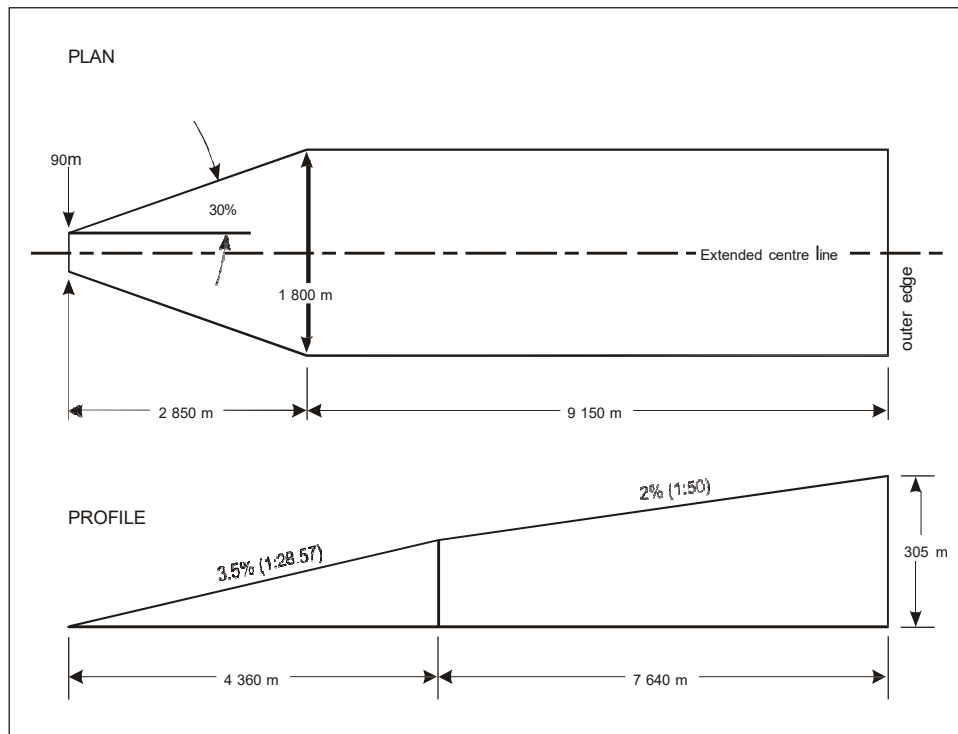
Figure A-2. Take-off climb surface for instrument FATO
