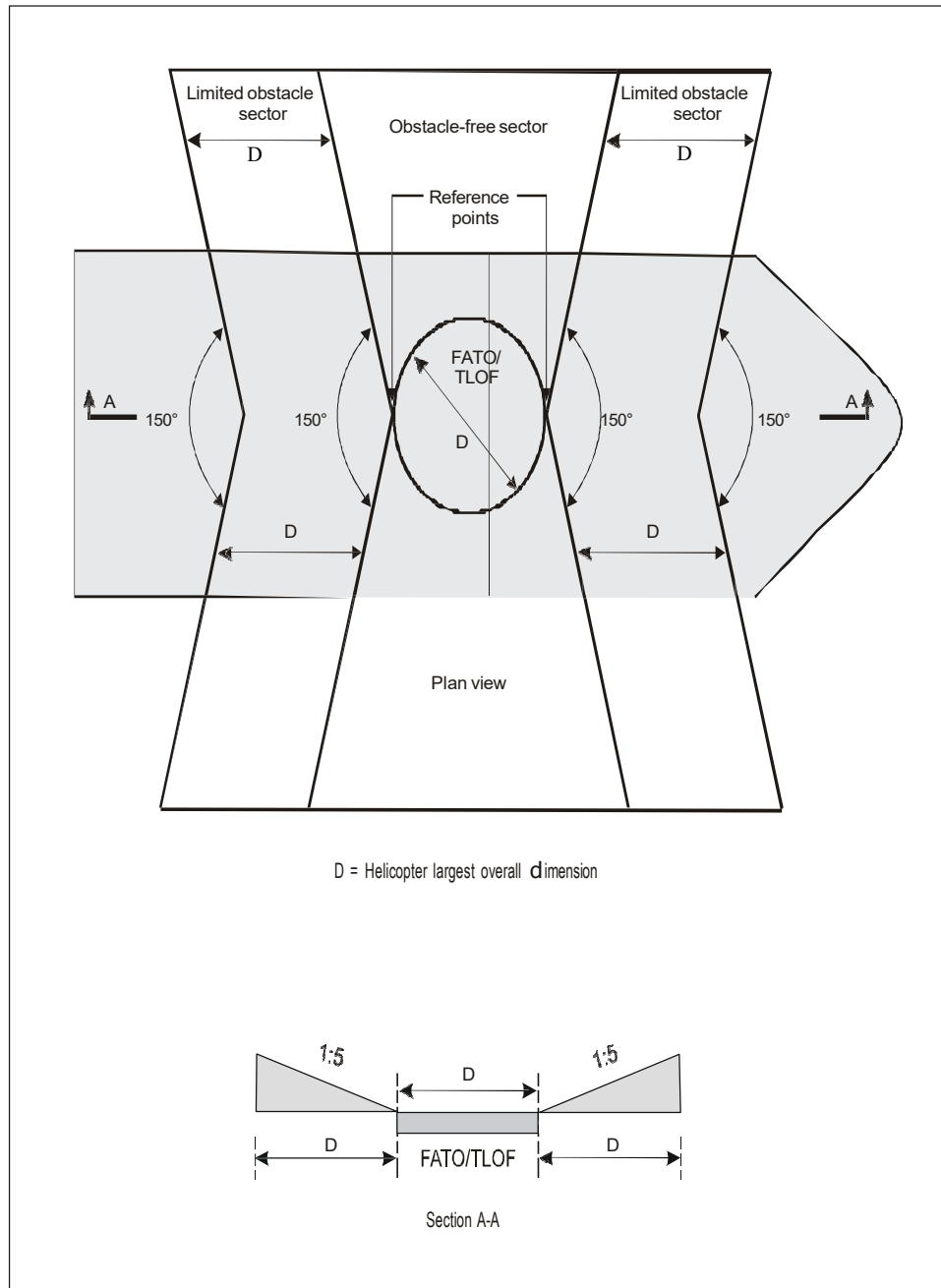
Figure 4-10. Amidship's location — shipboard heliport obstacle limitation surfaces
