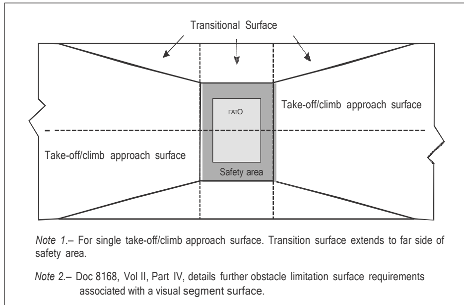
Figure A-5. Transitional surfaces for an instrument FATO with a non-precision and/or precision approach
