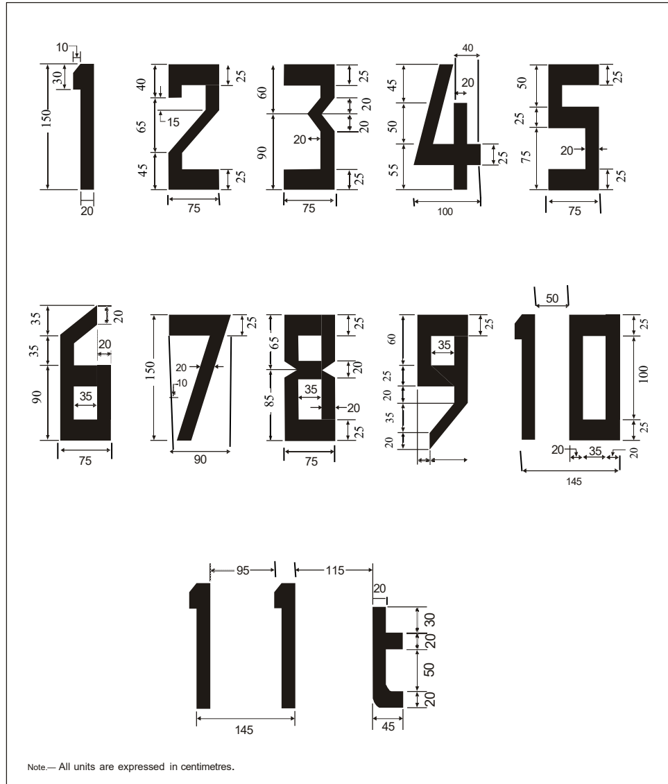
Figure 5-5. Form and proportions of numbers and letters
