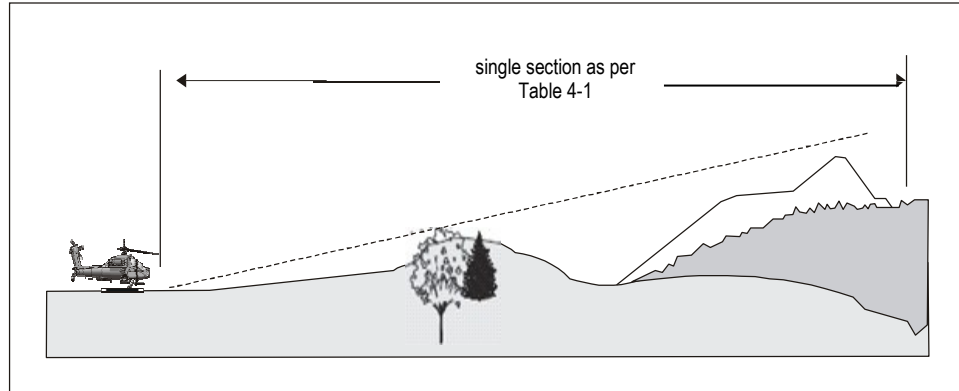
a) Approach and take-off climb surfaces – “A” slope profile - 4.5% design
