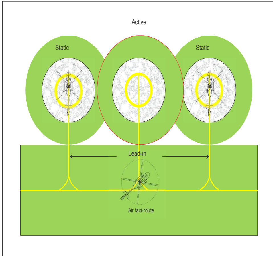
Figure 3-9. Turning stands (with air taxi-route) non-simultaneous use — inner stand active
