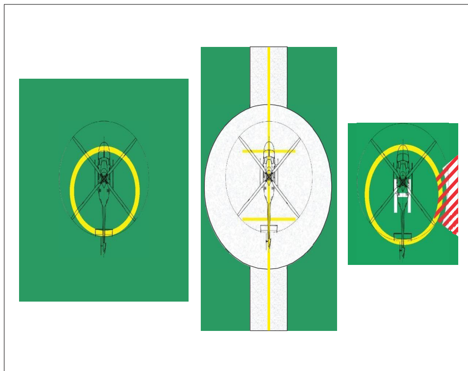
Figure 5-8. Multidirectional TDPC with no limitations (left) Unidirectional marking shoulder line with associated centreline (centre) Multidirectional TDPC with prohibited landing sector marking (right)
