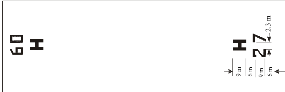
Figure 5-3. FATO designation marking and heliport identification marking for a runway-type FATO
