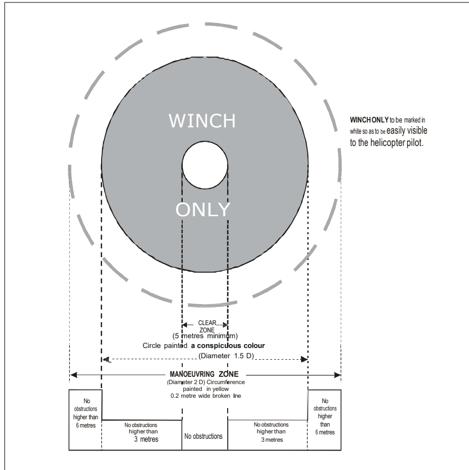
Figure 4-12. Winching area of a ship
