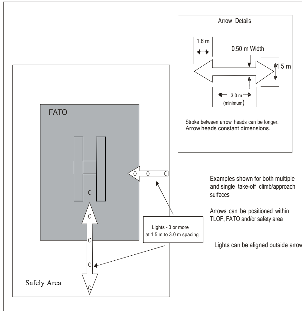
Figure 5-10. Flight path alignment guidance markings and lights
