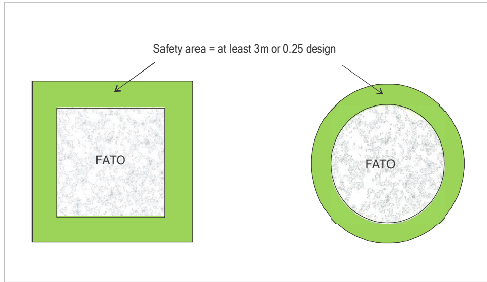
Figure 3-1. FATO and associated safety area
