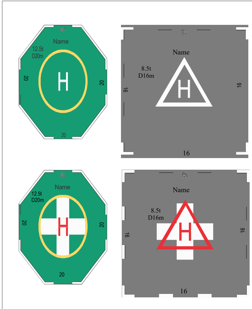
Figure 5-2. Heliport identification markings with TLOF and aiming markings for heliport and hospital heliport
