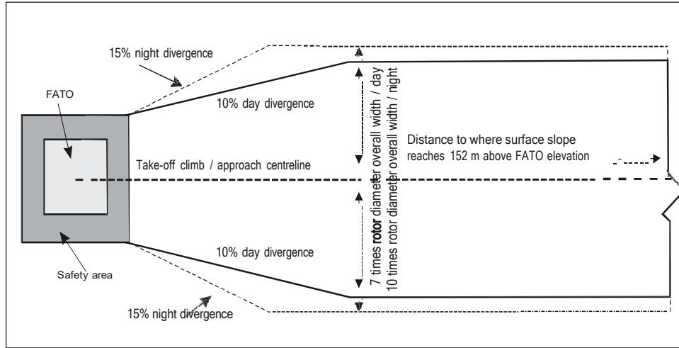
Figure 4-2. Take-off climb/approach surface width
