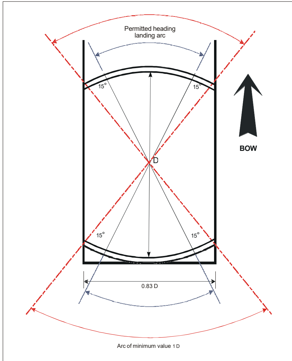
Figure 3-10. Shipboard permitted landing headings for limited heading operations
