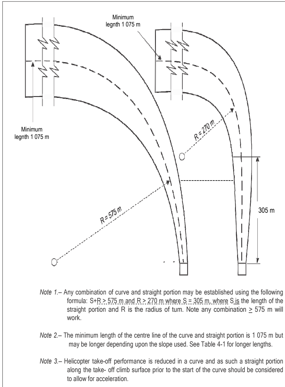
Figure 4-5. Curved approach and take-off climb surface for all FATOs
