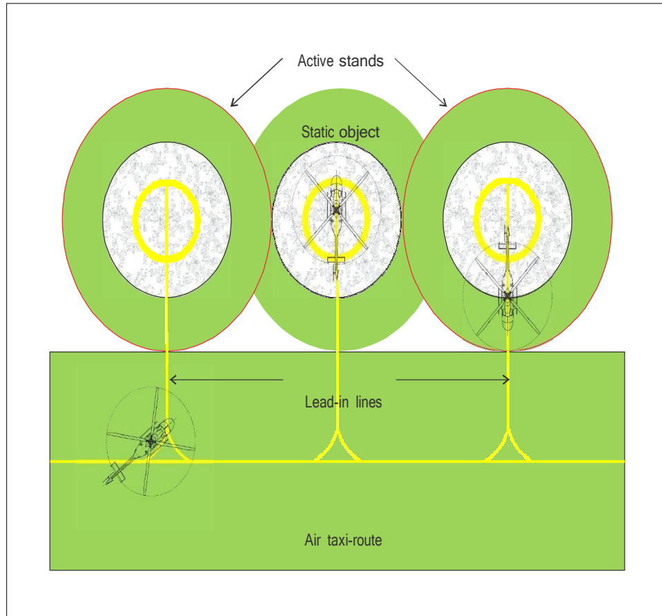
Figure 3-8. Turning stands (with air taxi -routes) non-simultaneous use — outer stands active
