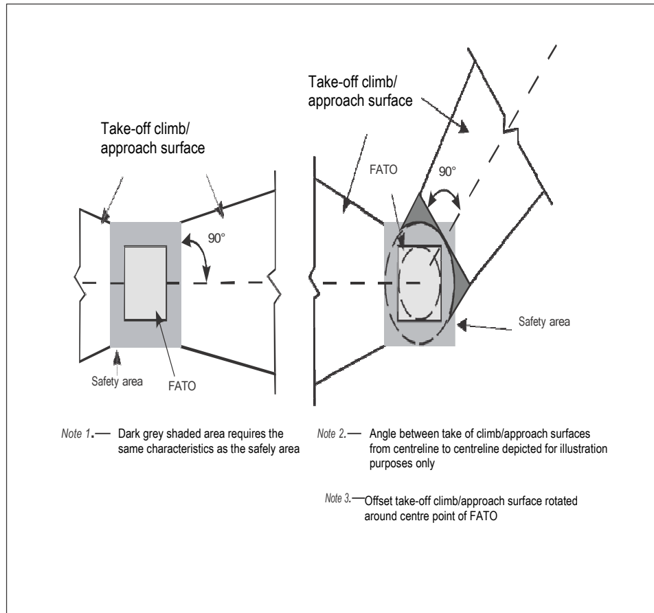
Figure 4-1. Obstacle limitation surfaces — take-off climb and approach surface
