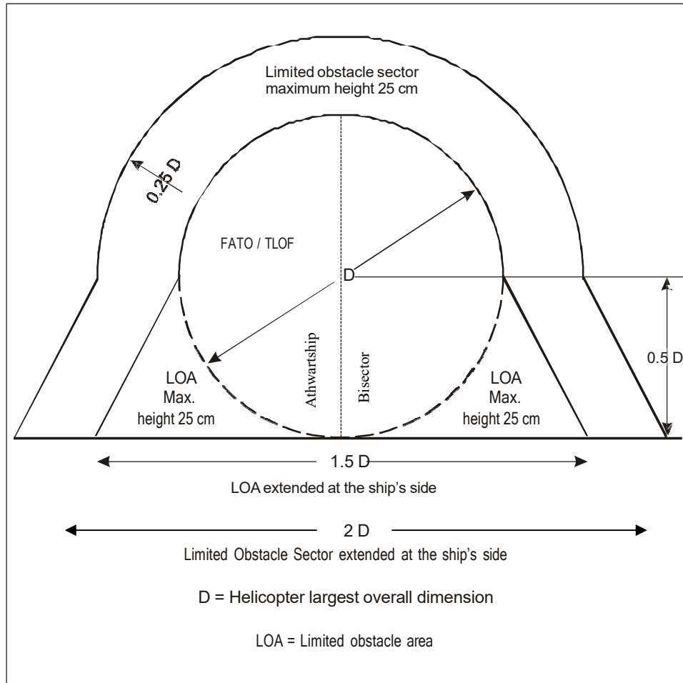
Figure 4-11. Ships-side non-purpose-built heliport obstacle limitation sectors and surfaces
