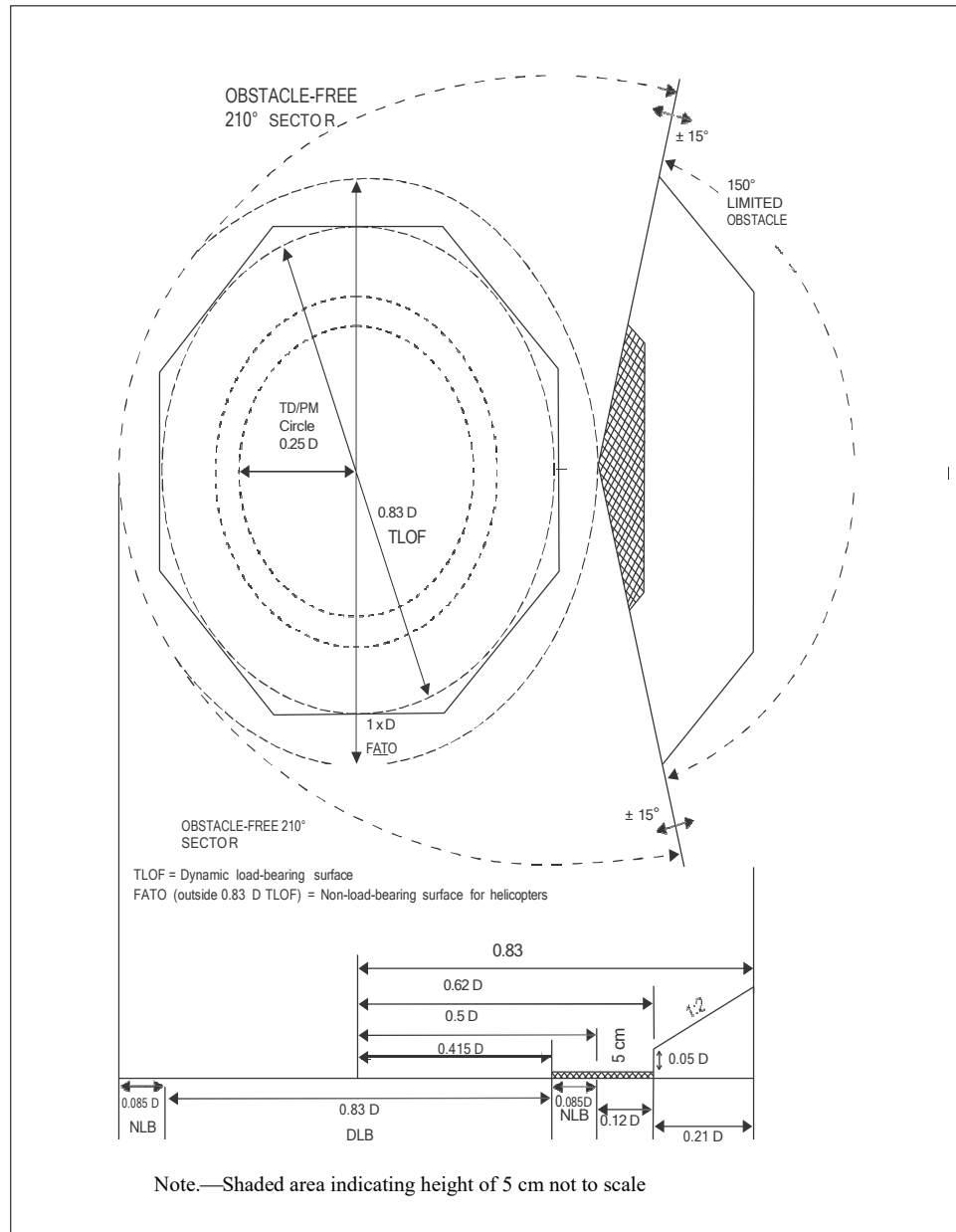
Figure 4-9. Helideck obstacle limitation sectors and surfaces for a TLOF of 0.83 D and larger
