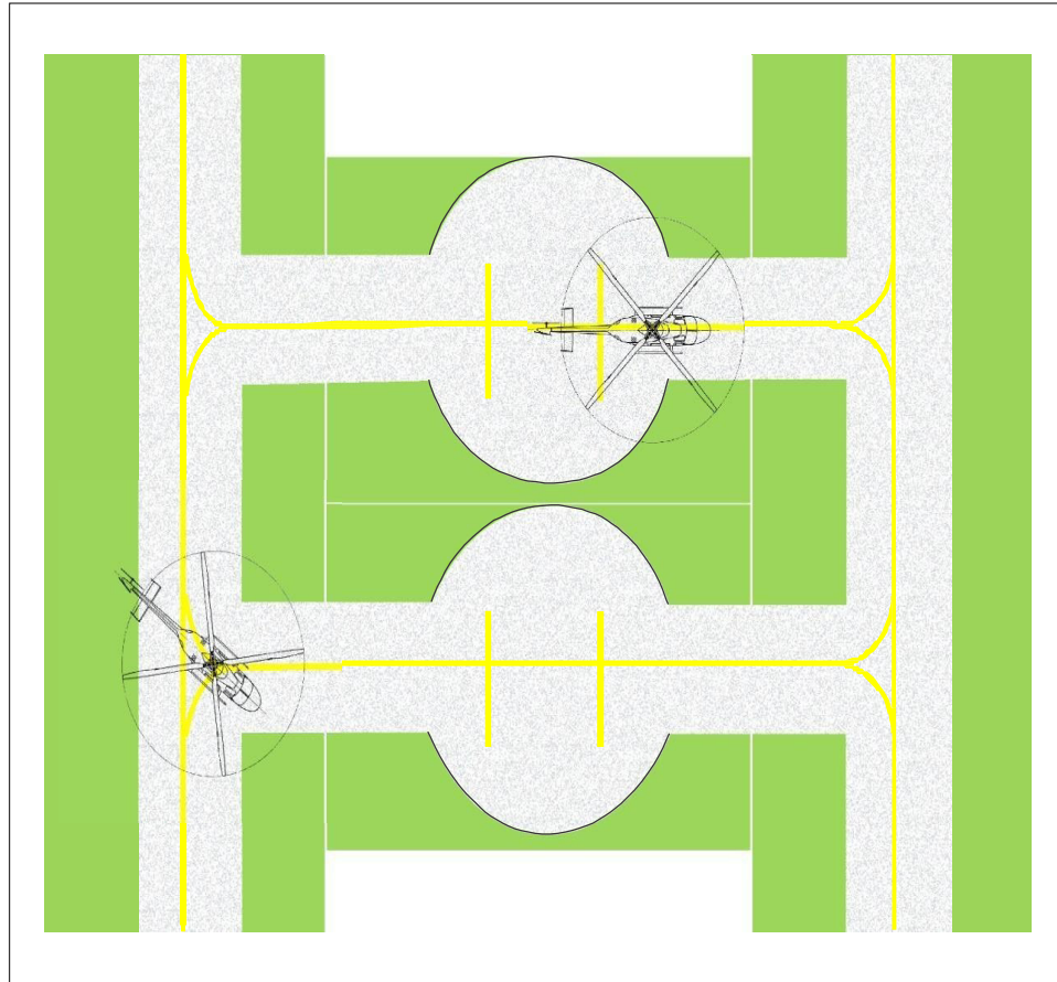
Figure 3-6. Ground taxi-through stands (with taxiway/ground taxi-route) simultaneous use
