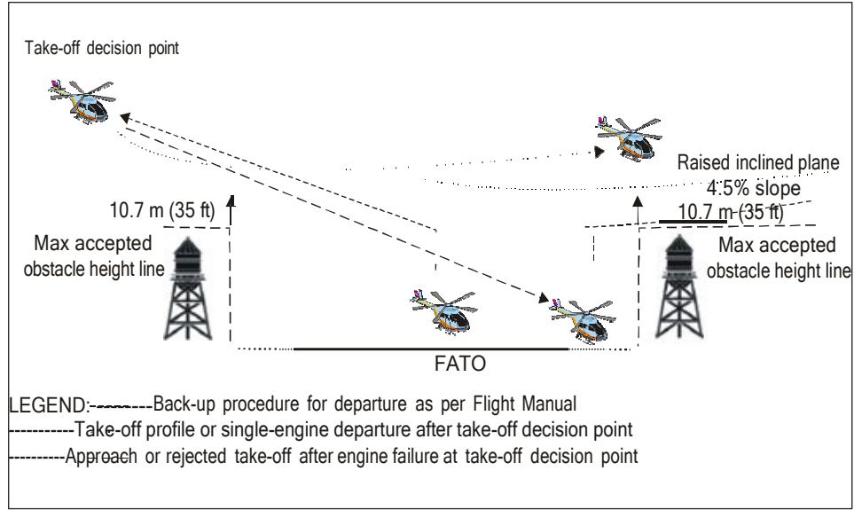
Figure 4-4. Example of raised inclined plane during operations in performance class 1
