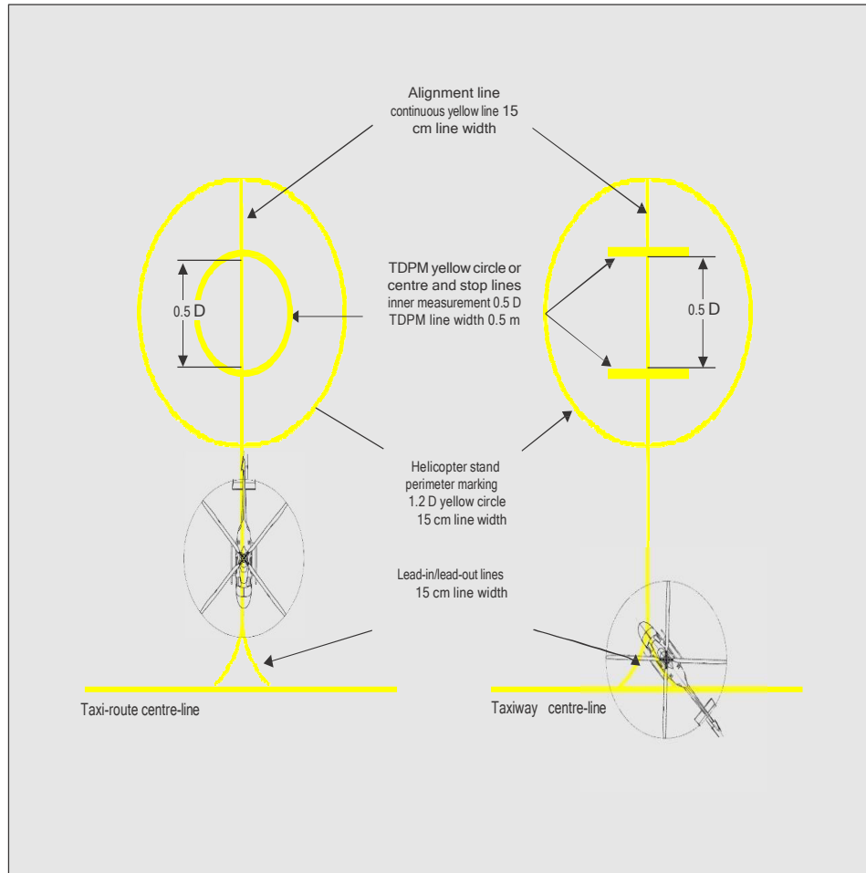
Figure 5-9. Helicopter stand markings
