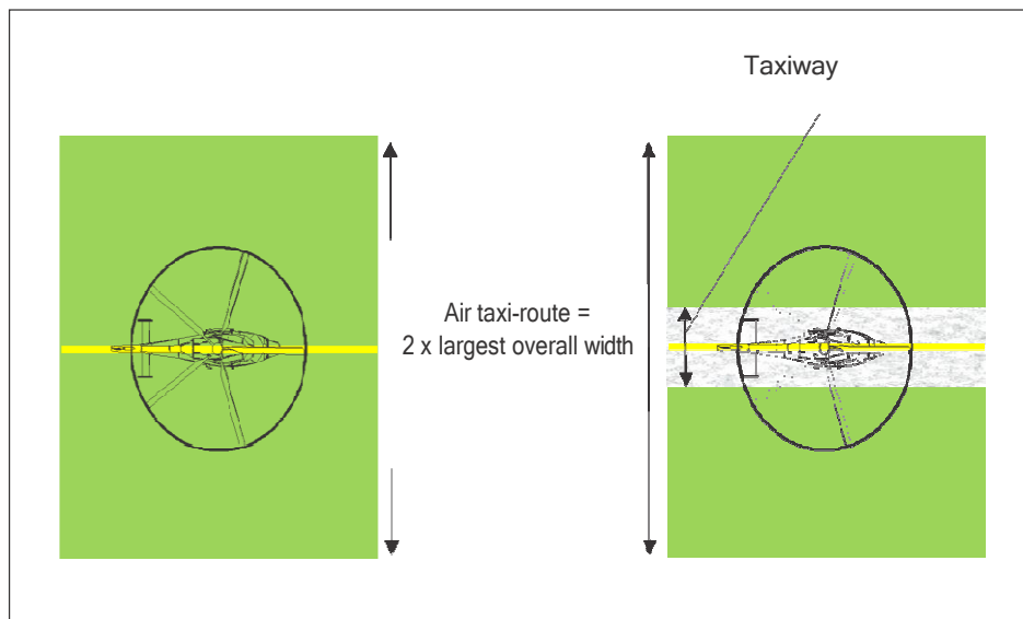
Figure 3-4. Helicopter air taxi-route and combined air taxi-route/taxiway
