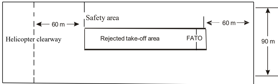
Figure A-1. Safety area for instrument FATO
