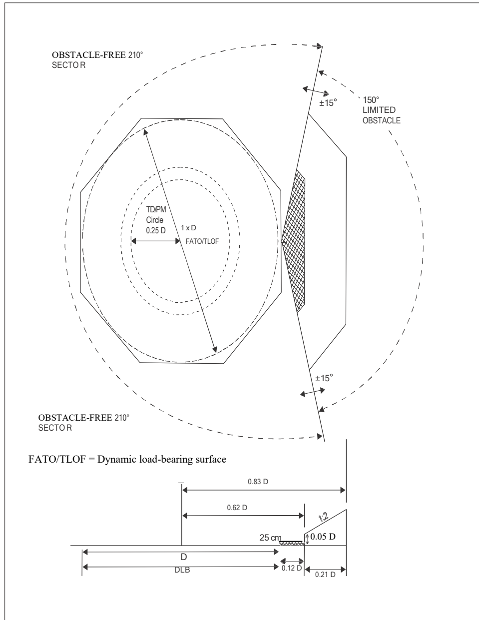
Figure 4-8. Helideck obstacle limitation sectors and surfaces for a FATO and coincidental TLOF of 1 D and larger
