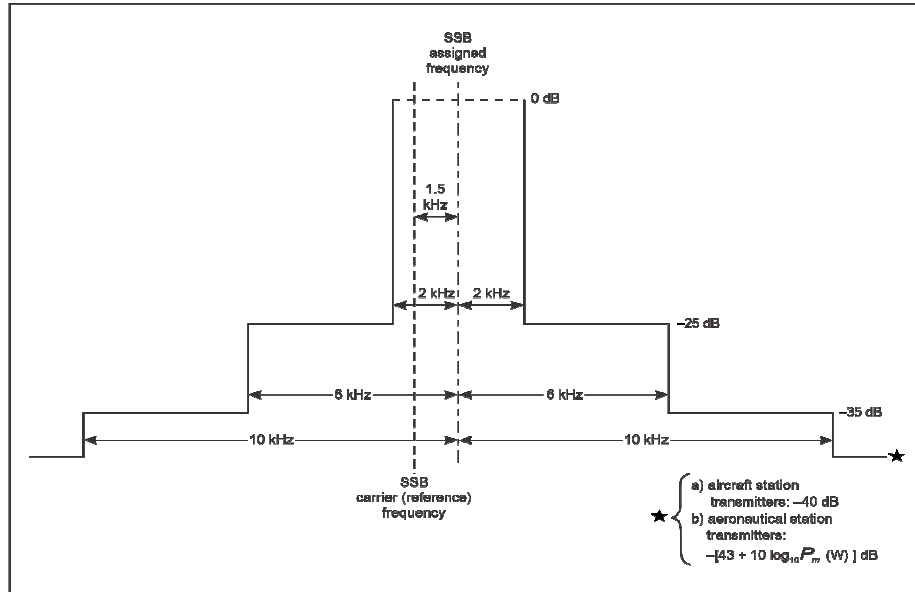
Figure 2-1. Required spectrum limits (in terms of mean power) for aircraft station transmitter types and for aeronautical station transmitters first installed before 1 February 1983
