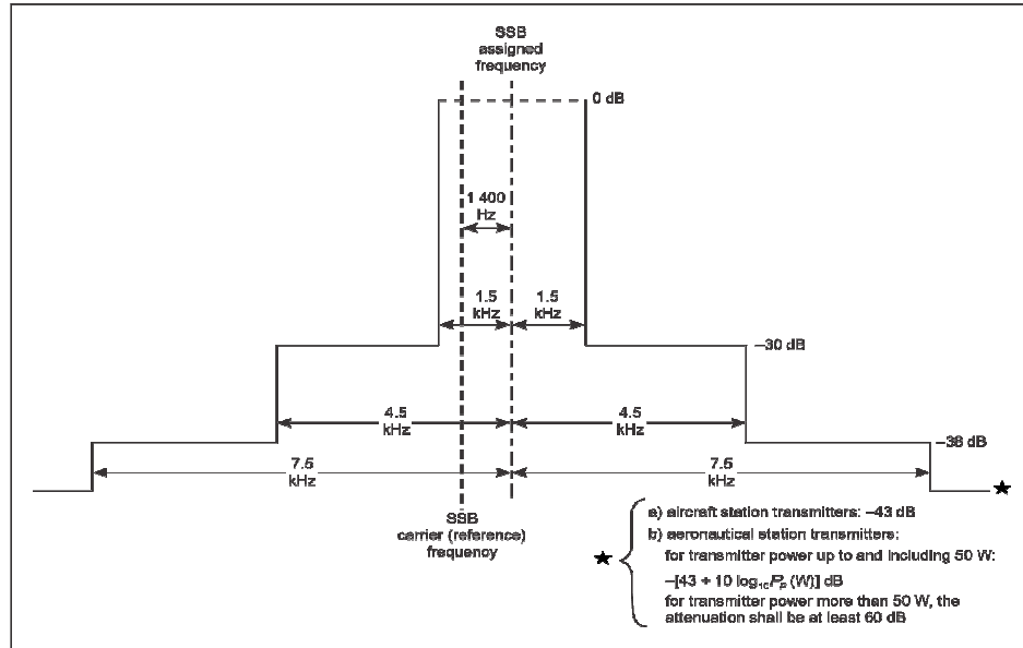
Figure 2-2. Required spectrum limits (in terms of peak power) for aircraft station transmitters first installed after 1 February 1983 and aeronautical station transmitters in use after 1 February 1983
