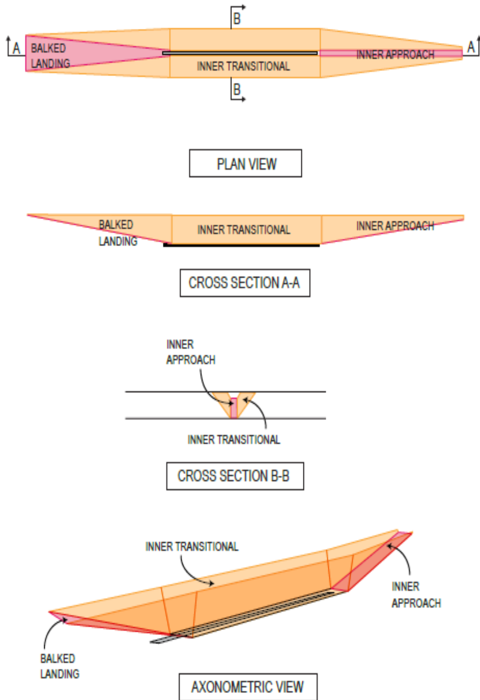
Figure 4-3 Obstacle free zone on a precision approach runway
