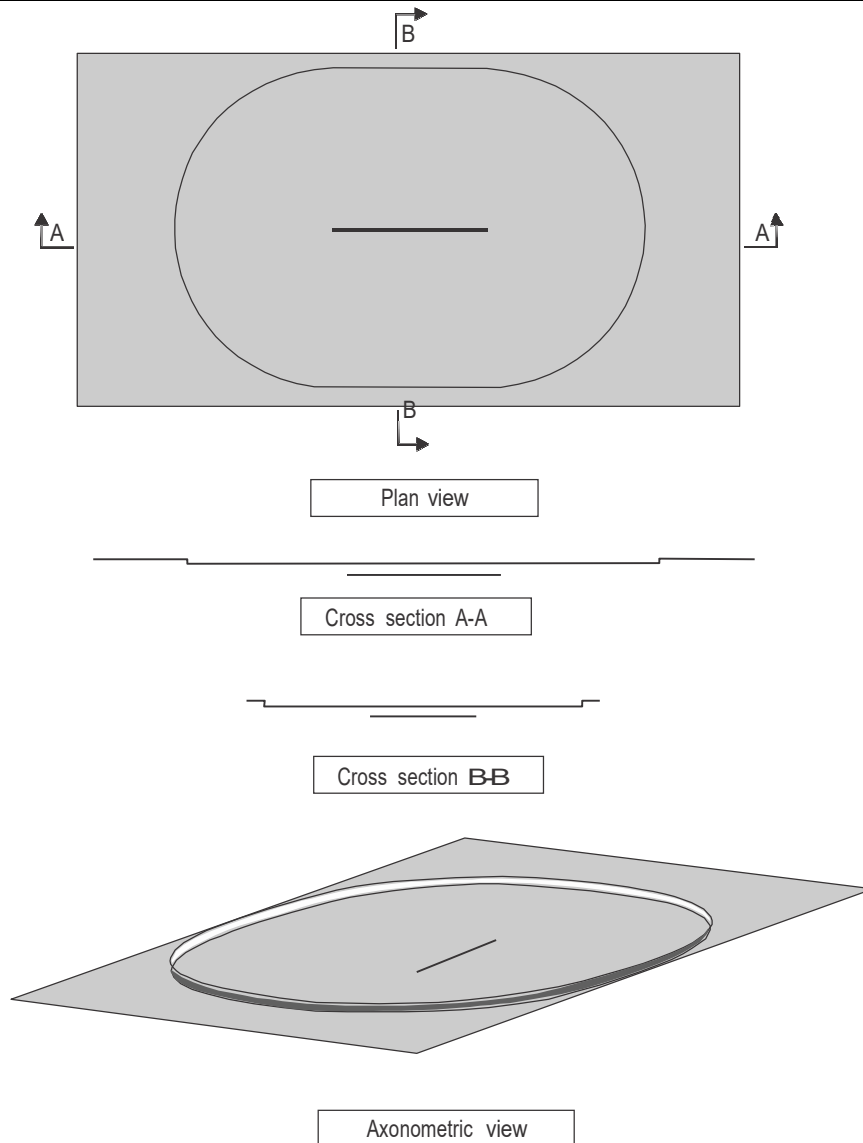
Figure 4-5. Surface for straight-in instrument approaches
