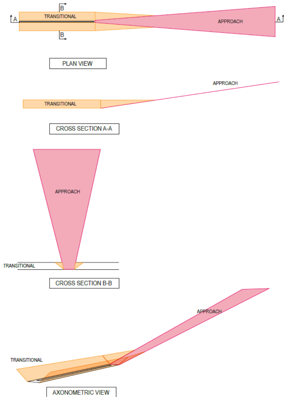
Figure 4-1. Approach surface and transitional surfaces
