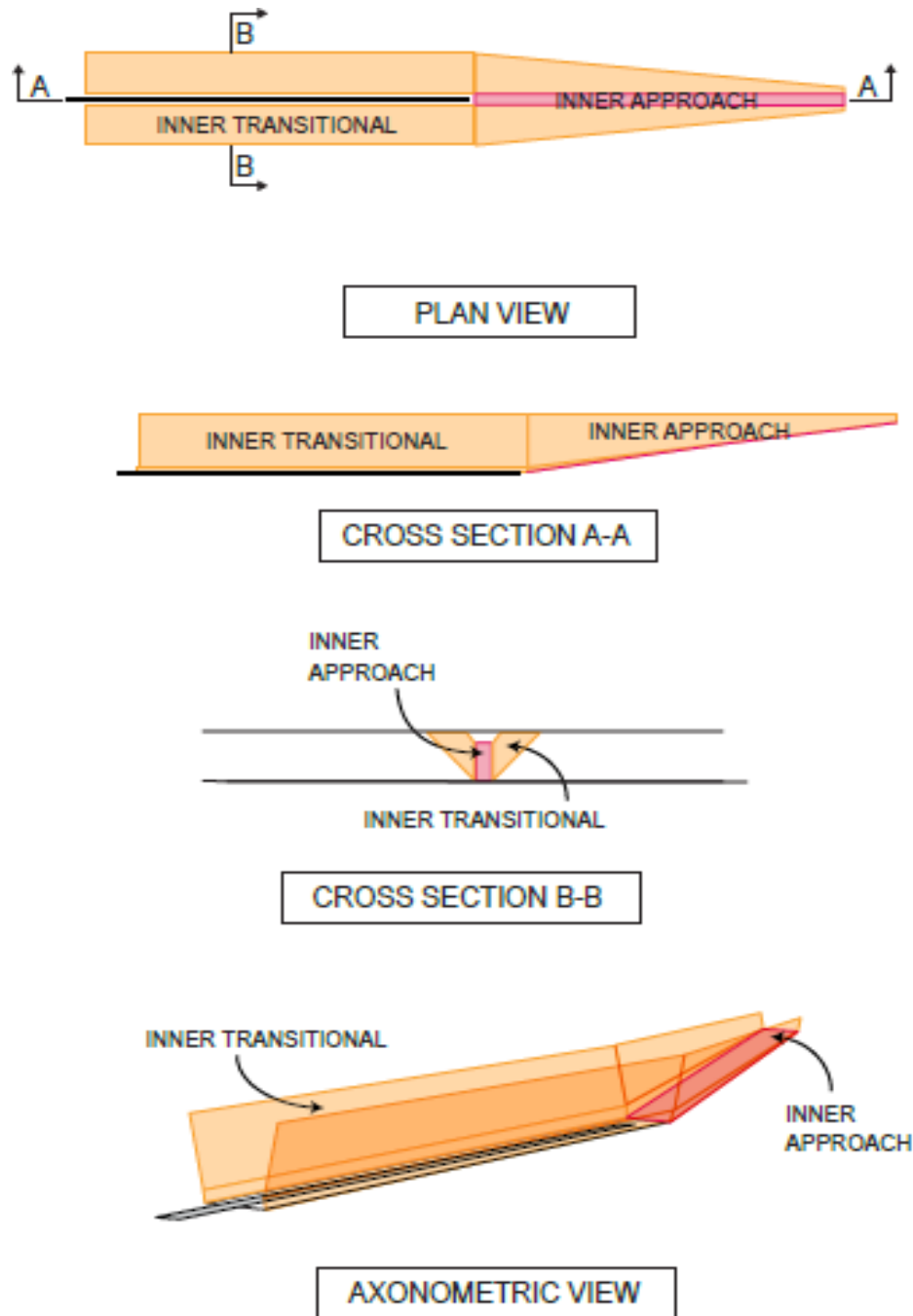
Figure 4-2 Inner approach and inner transitional surfaces on a non-precision approach runway
