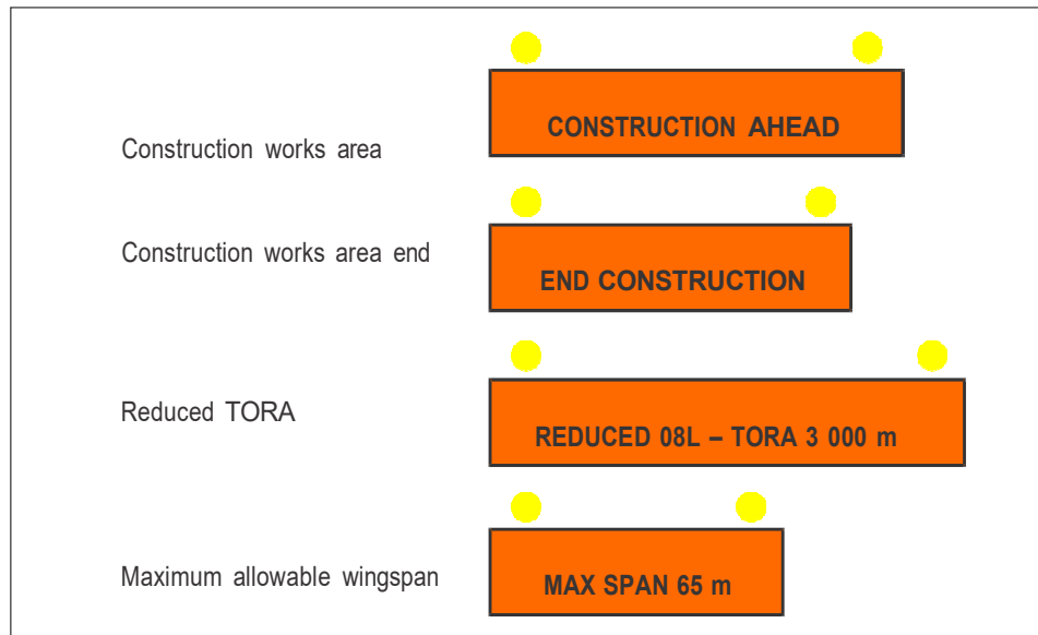
Figure 7-3. Examples of unserviceability signs
