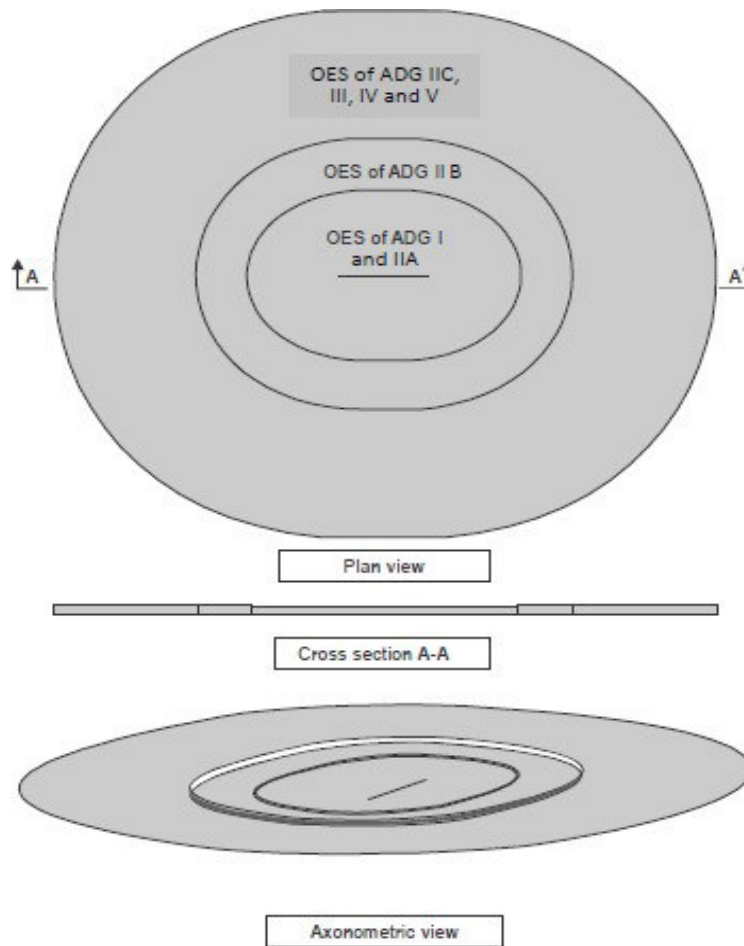
Figure 4-4. Horizontal surface
