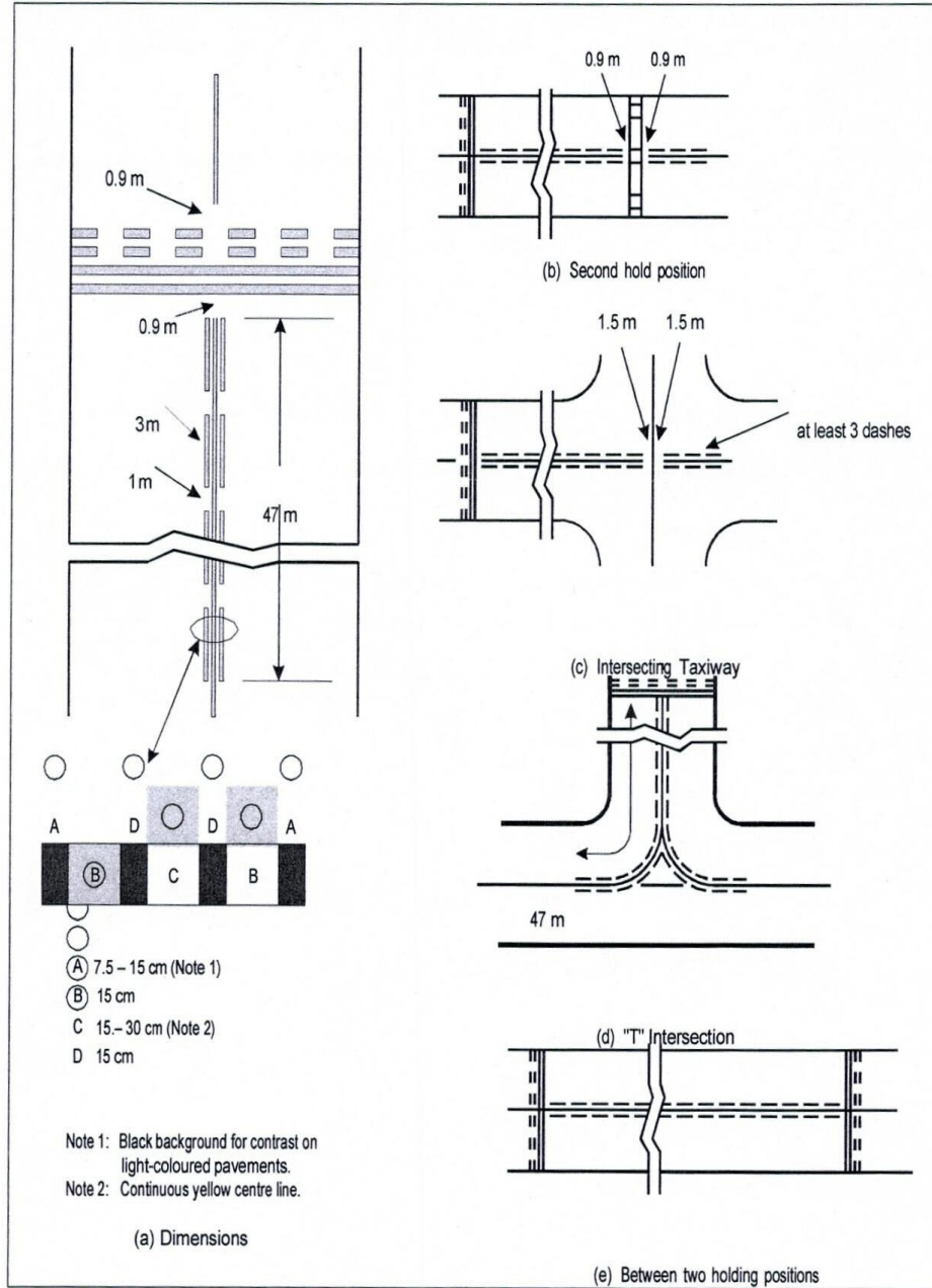
Figure 5-7. Enhanced taxiway centre line marking
