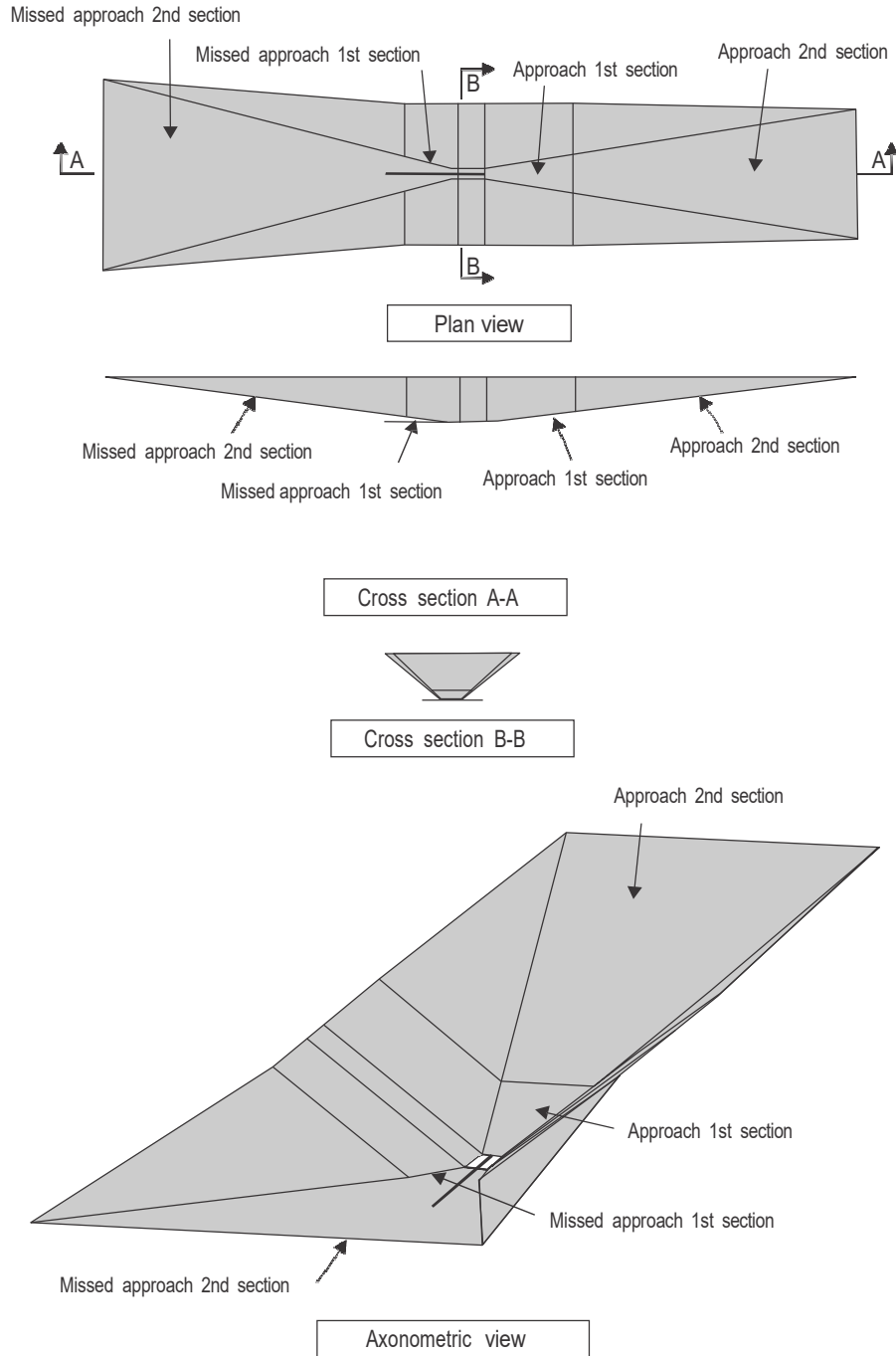
Figure 4-6. Surface for precision approaches
