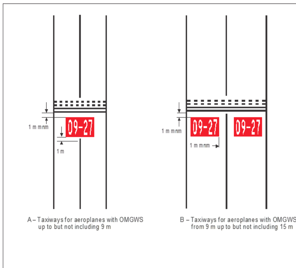
Figure 5-10. Mandatory instruction marking
