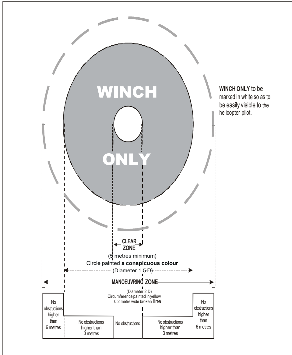
Figure 4-712. Winching area of a ship
