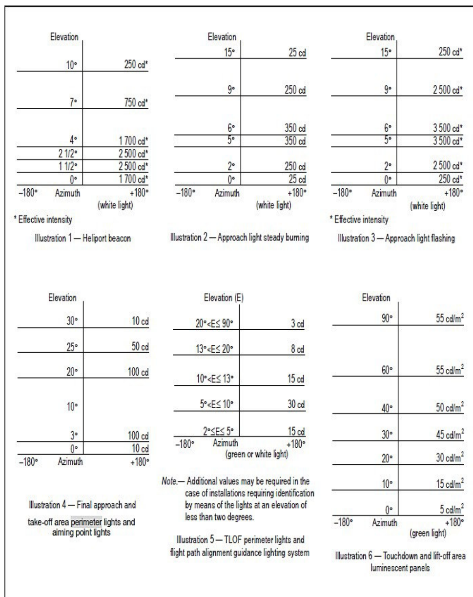
Figure 5-12. Isocandela diagrams
