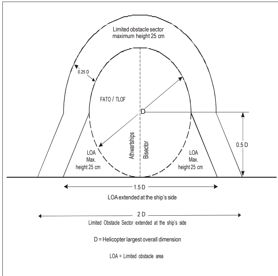
Figure 4-611. Ships-side non-purpose-built heliport obstacle limitation sectors and surfaces
