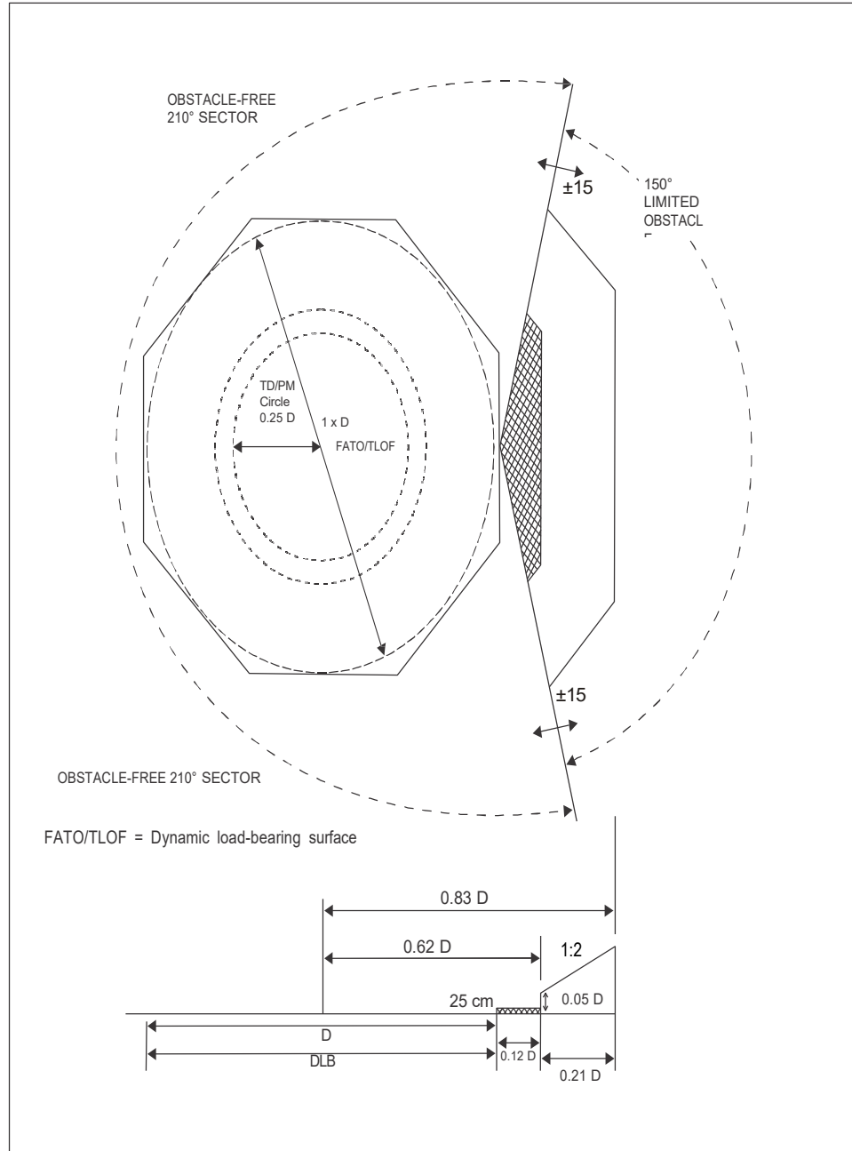
Figure 4-38. Helideck obstacle limitation sectors and surfaces for a FATO and coincidental TLOF of 1 D and larger
