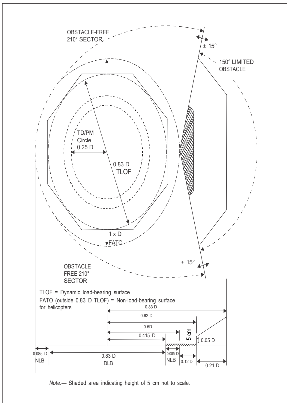
Figure 4-49. Helideck obstacle limitation sectors and surfaces for a TLOF of 0.83 D and larger
