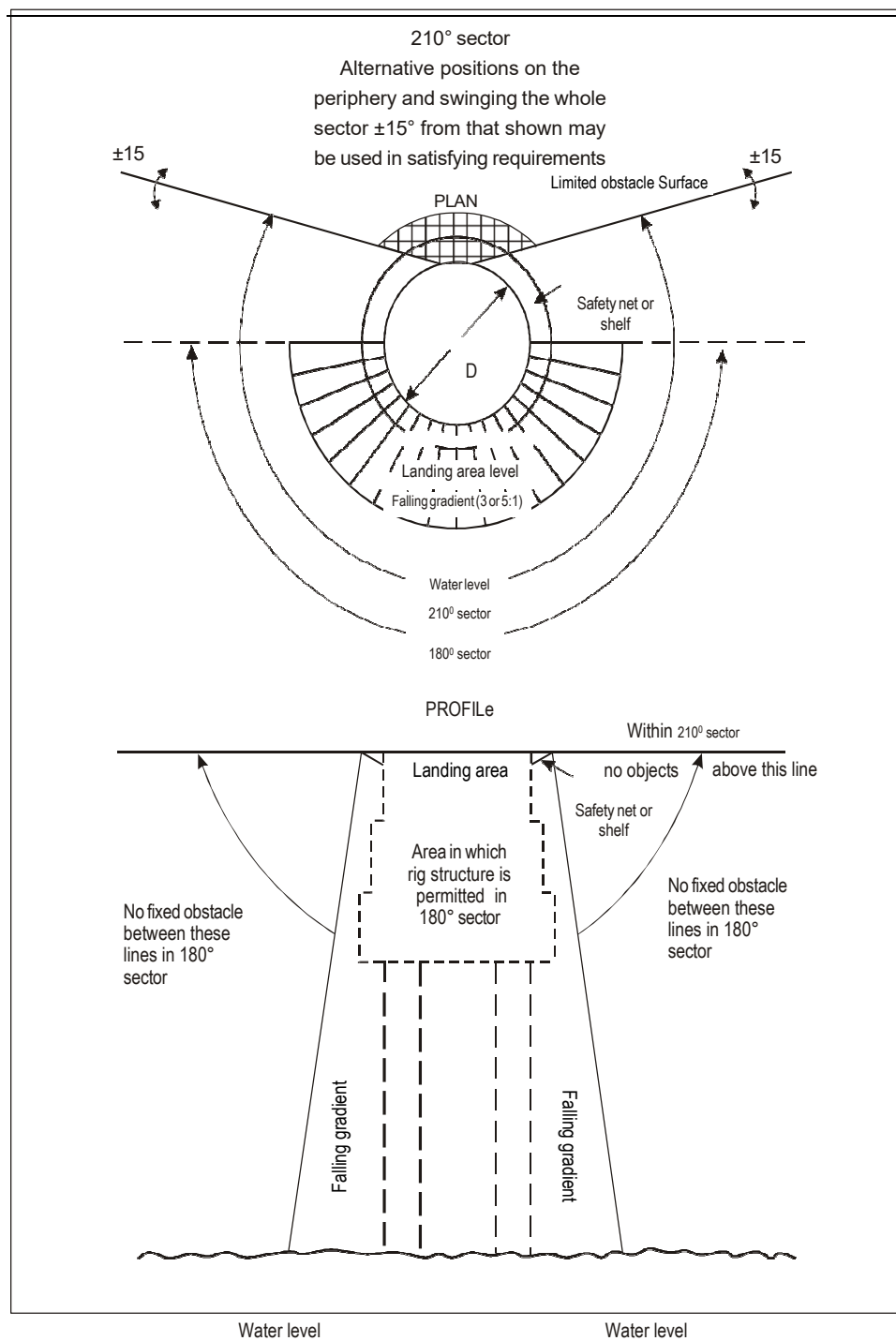
Figure 4-27. Helideck obstacle-free sector
